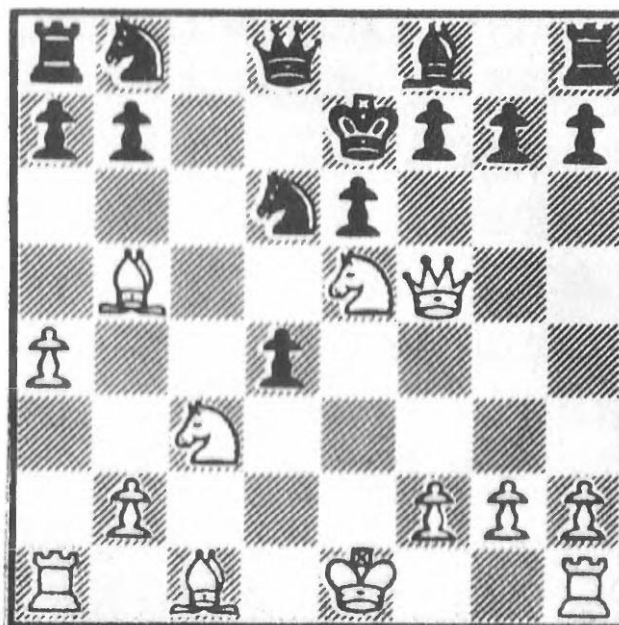
128 After 11...Ke7
